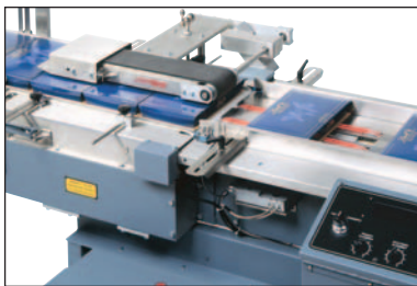
Synchronic Overhead Belt Infeed
